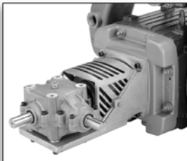
Direct Mount Cast Aluminum and Right Angle Gearbox Drive Assembly
